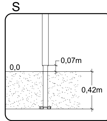
S Sunken Foundation 8077966 8105667
